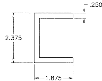
7 SIDE CHANNEL
