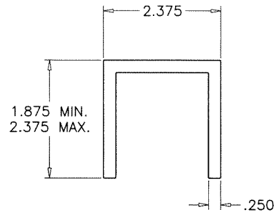
1 TOP CHANNEL
