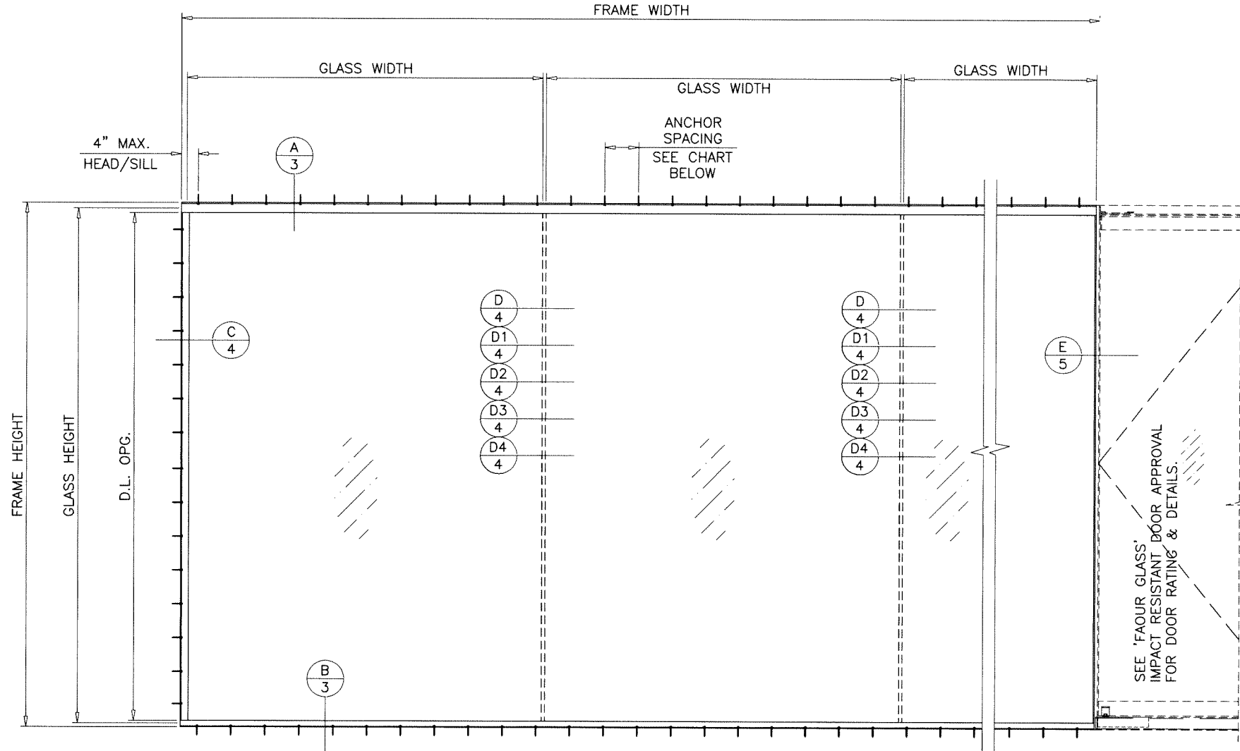
TYPICAL ELEVATIONS
