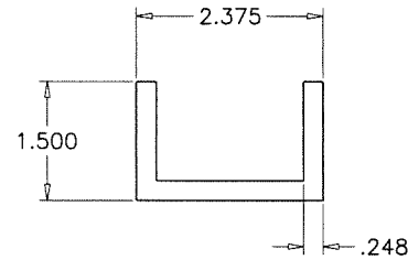
2 BOTTOM CHANNEL
